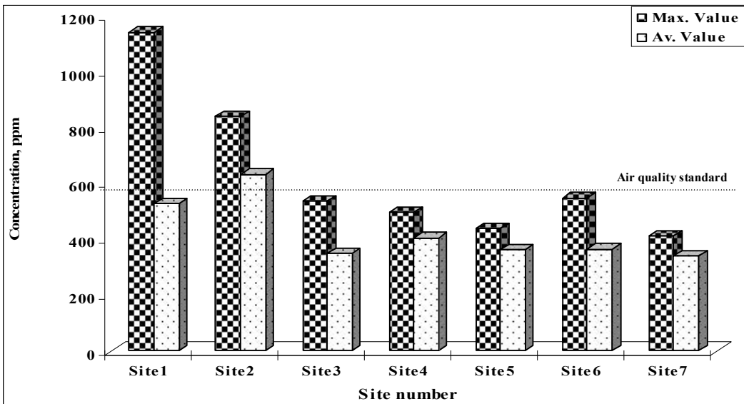
Fig. (6): Variation of Maximum and Average Concentration of CO 2 in Gerga Sugar Factory (March 2007)
