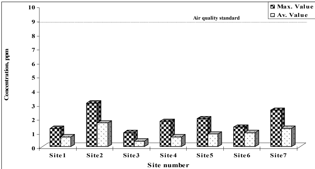
Fig. (5): Variation of Maximum and Average Concentration of CO in Gerga Sugar Factory (March 2007)
